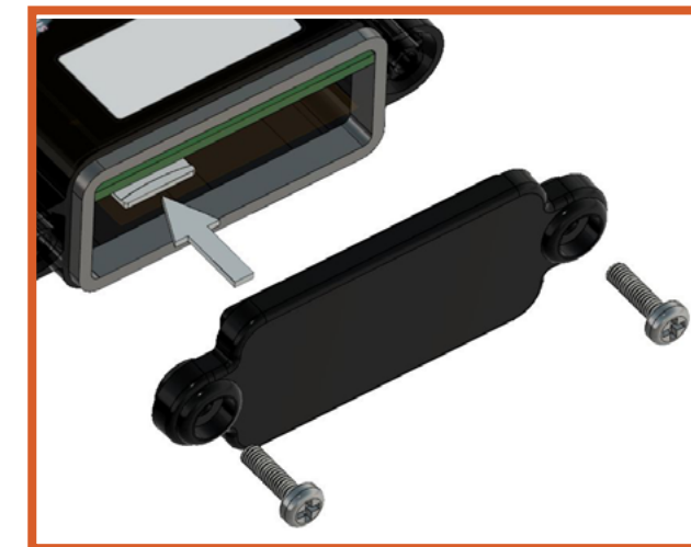
Micro SD card ejection
